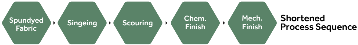
Spunshades Process (5 Stages) vs Conventional Process (8 Stages)
